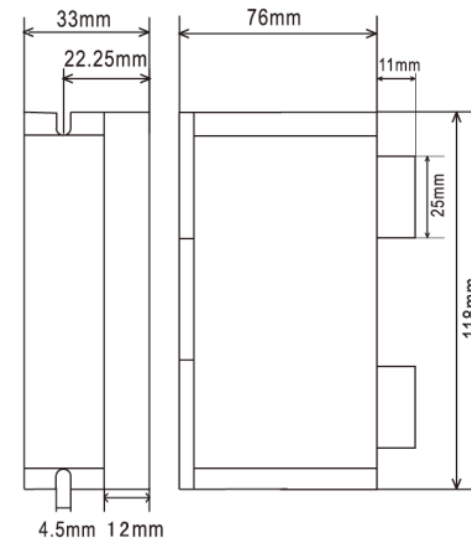
Figure 2: Mechanical specifications
