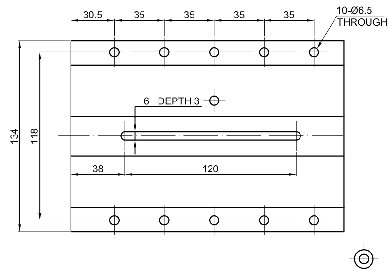
B VIEW BOTTOM OF SHELL
