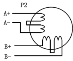
Figure 7: 8-lead motor series connections
