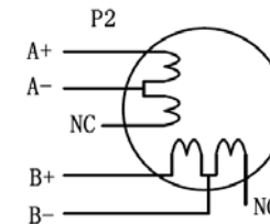
Figure 4: 4-lead Motor Connections
