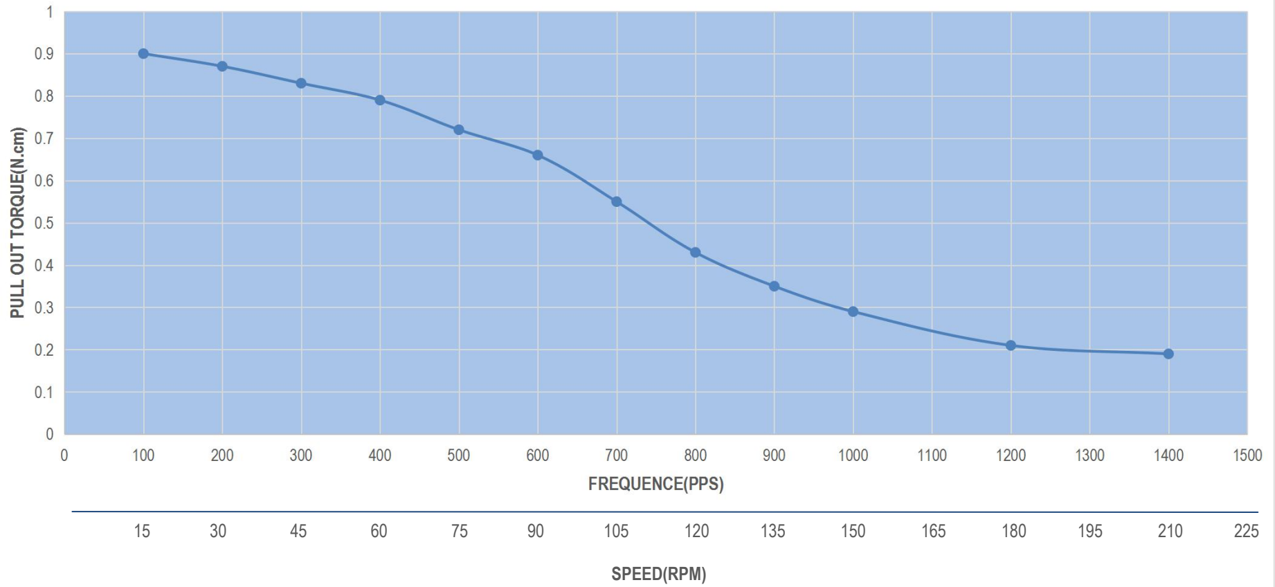
PULL OUT TORQUE(0.18A/P 24V HALF STEP)
