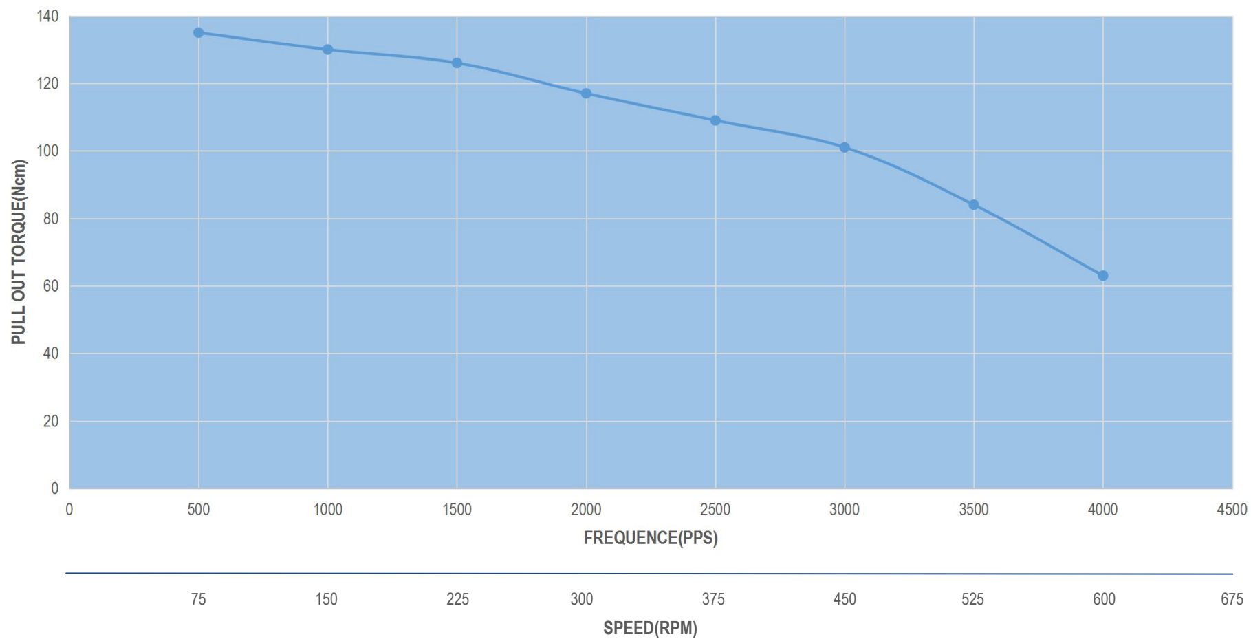
24HS39-3008D PULL OUT TORQUE(3A/P 36V HALF STEP)
