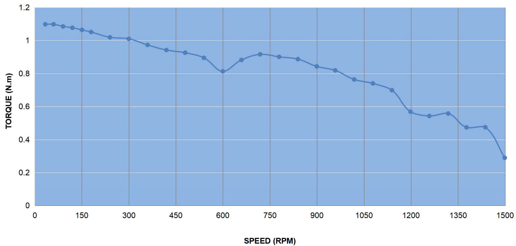
PULL OUT TORQUE CURVE OF 23HT32-5503S
