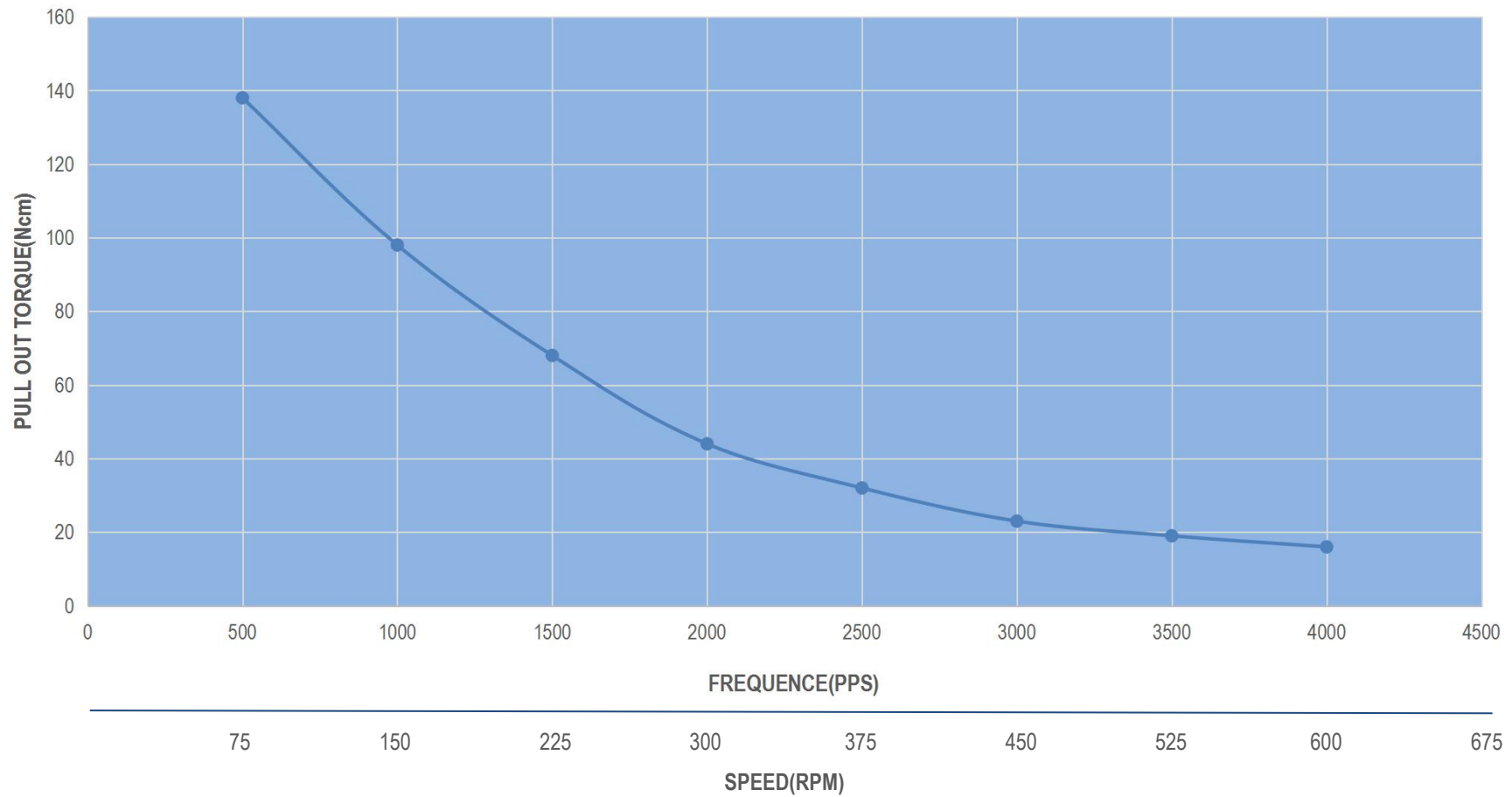
23HS30-2804S PULL OUT TORQUE(2.8A/P 24V HALF STEP)
