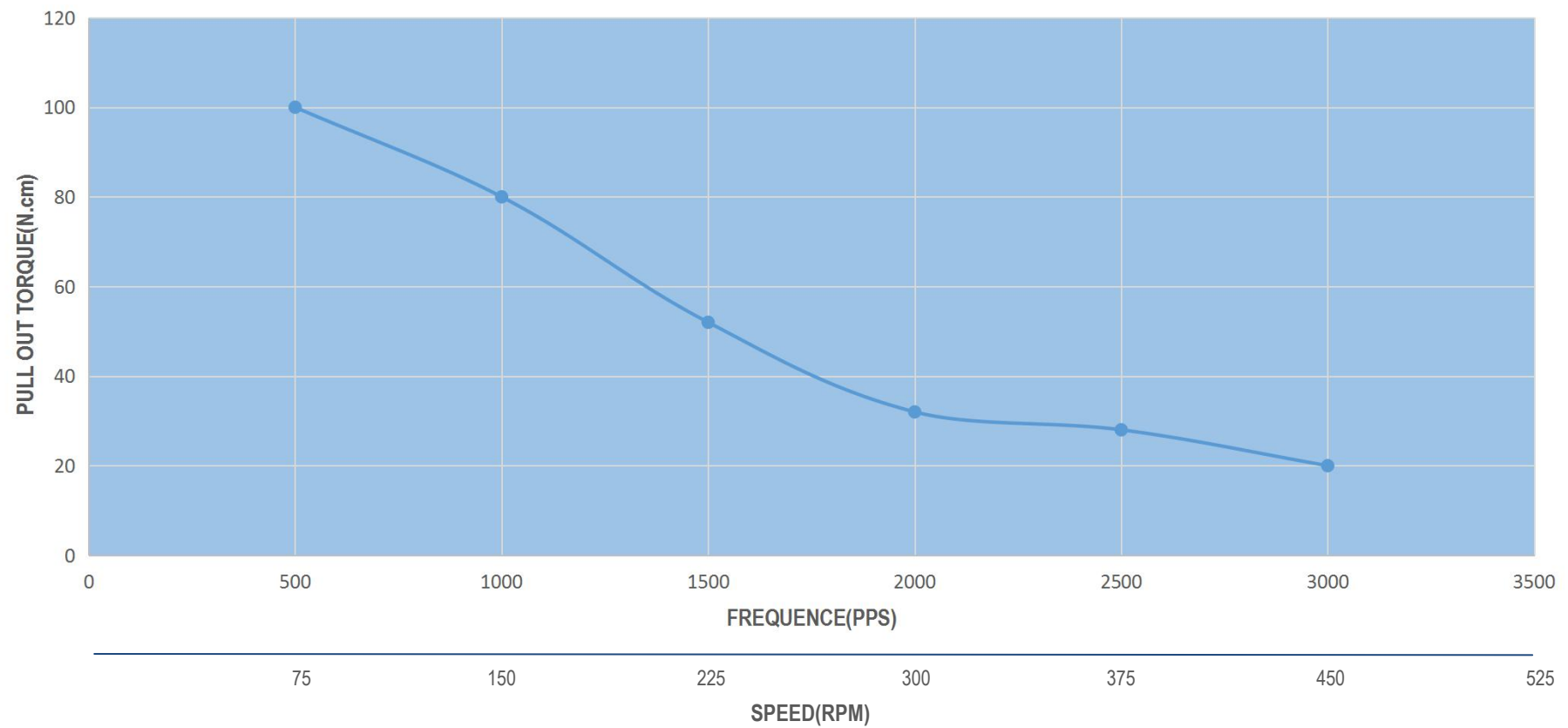
23HS22-1504S PULL OUT TORQUE (1.5A/PHASE 24V CONSTANT CURRENT HALF STEP)
