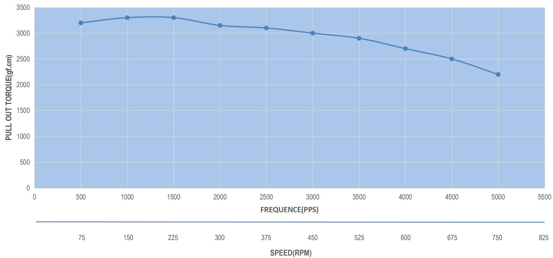
17HS19-1684S1 PULL OUT TORQUE (1.68A/PHASE 24V CONSTANT CURRENT HALF STEP)
