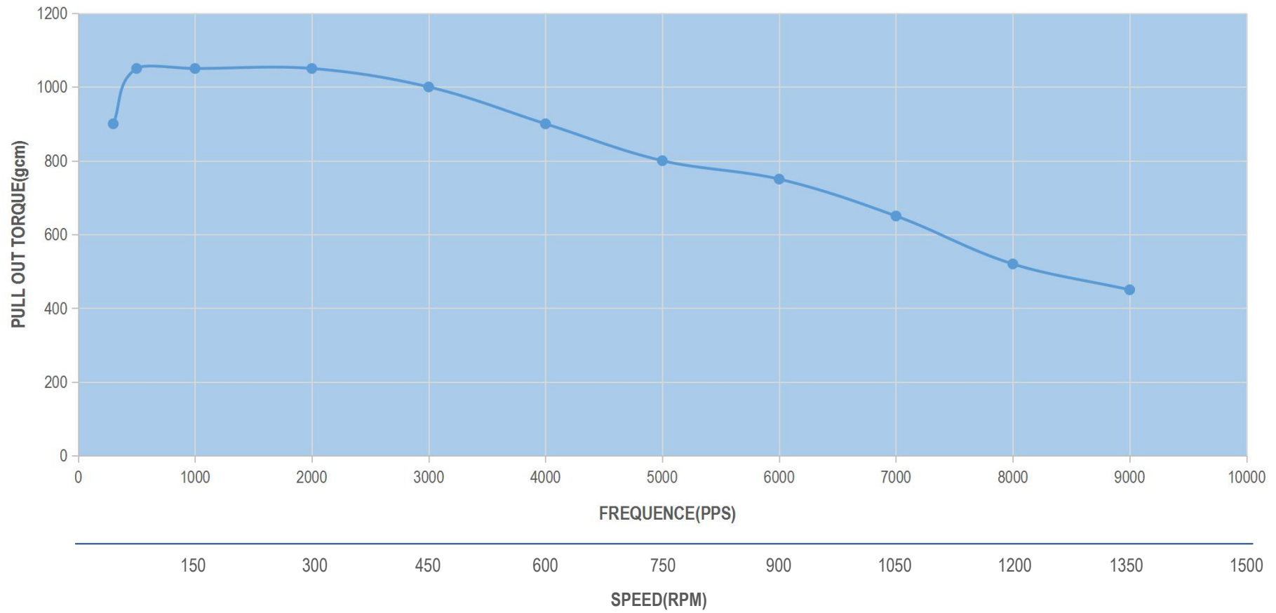
17HS10-0704S PULL OUT TORQUE(0.7A/P 24V HALF STEP)
