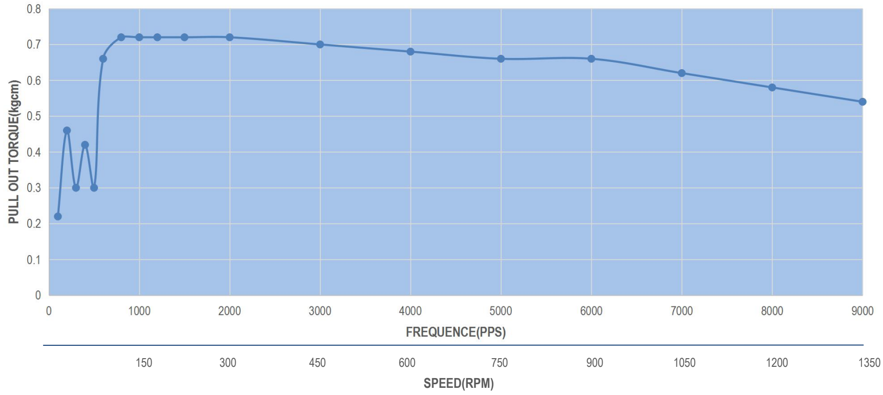
14HR08-0654S-D-Y4 PULL OUT TORQUE(0.8A/P 24V HALF STEP )
